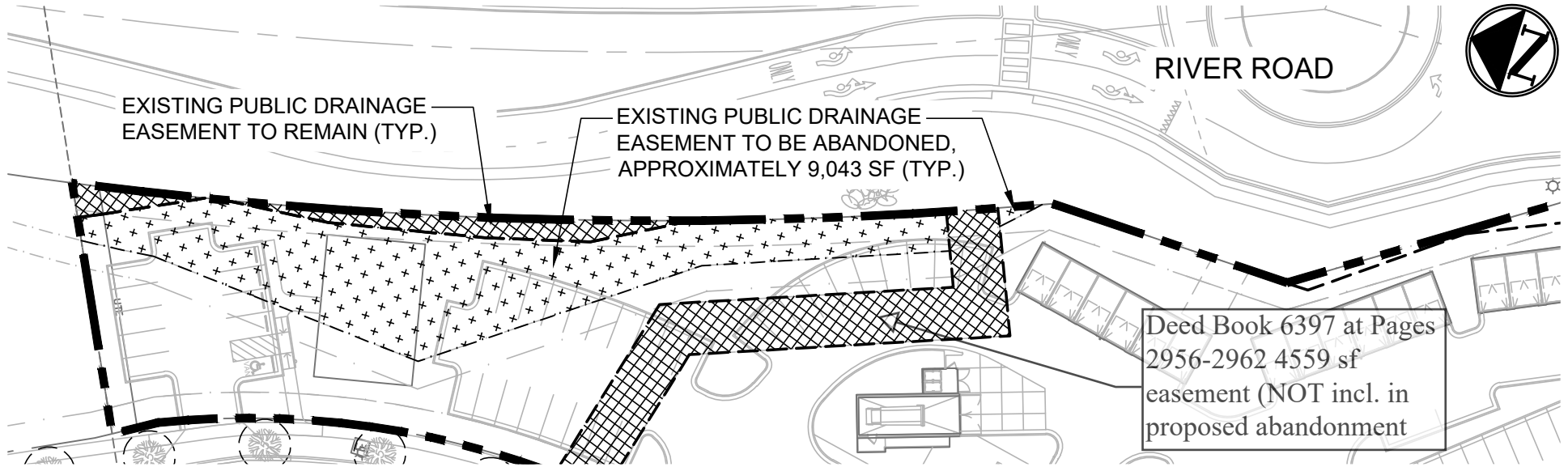
MX1C PLAN
